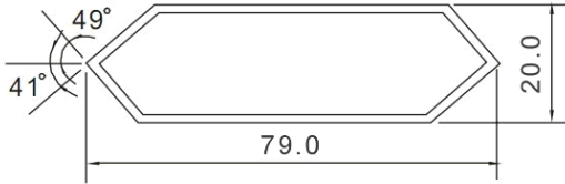
BL-SE700SEGMENT Dimension
