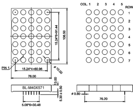
BL-M40X571 Series
