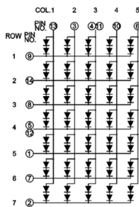
BL-M40A571
