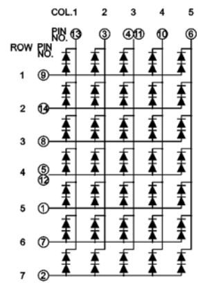
BL-M40B571
